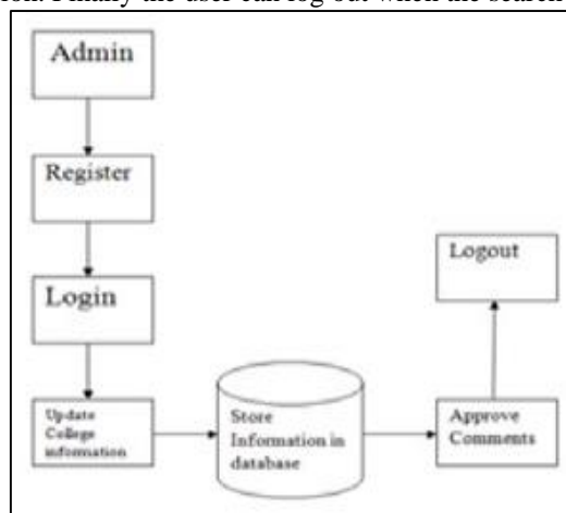
Fig. 2: Block diagram of admin side
