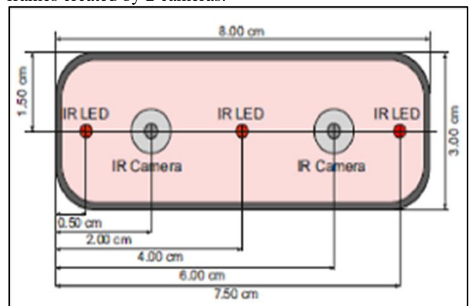
Fig. 2: Construction of Leap Motion Controller
