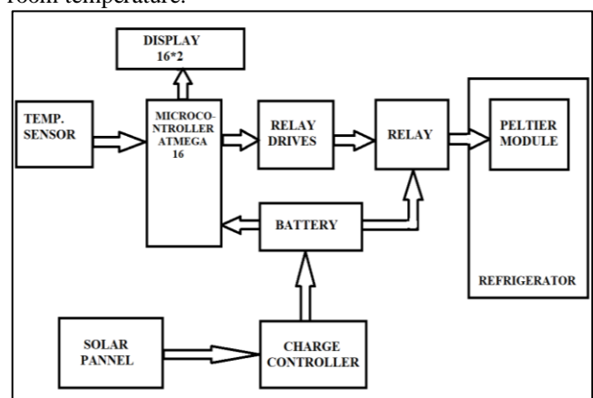
Fig. 1: Block diagram solar based refrigeration system
