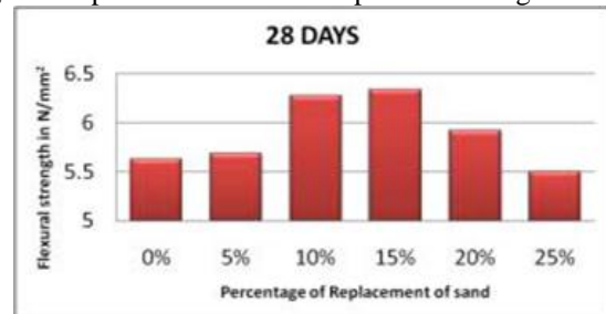
Fig. 2: Graph of variation of Flexural strength value at 28 days
