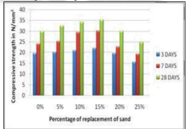
Fig. 1: Graph of variation of compressive strength with age
