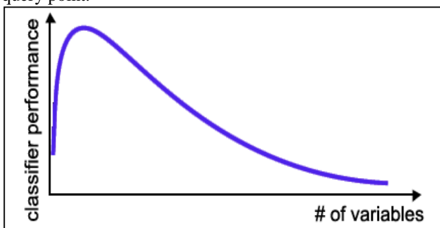
Fig 1. Curse of Dimensionality
