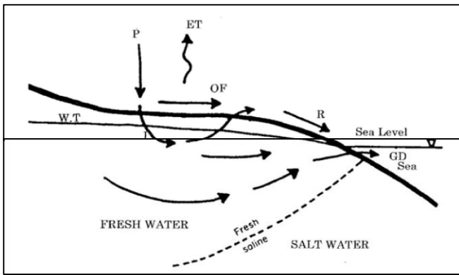
Figure 1: Conceptual Model of the Water Balance in a Coastal Watershed To assess the impacts of potential climate change on fresh groundwater resources, we should focus on changes in groundwater recharge and sea level rise on the loss of fresh groundwater resources in water resources stressed coastal aquifers.
