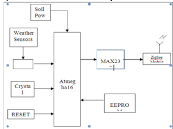
Fig. 1: Transmitter Section of the Wireless Monitoring System.
