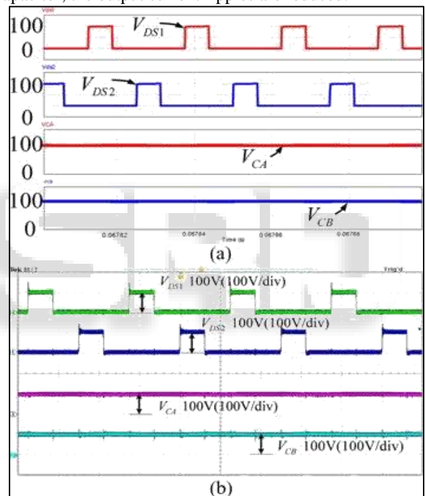
Fig. 6: Waveforms of the voltage stress of V_{DS1} , V_{DS2} , V_{CA} , and V_{CB}
