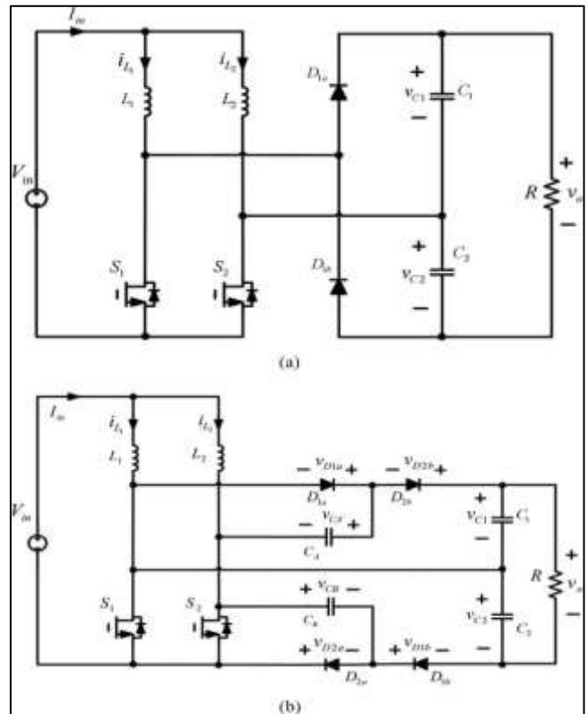
Fig. 1: Configurations of (a) two-phase interleaved boost converter (b) the proposed converter
