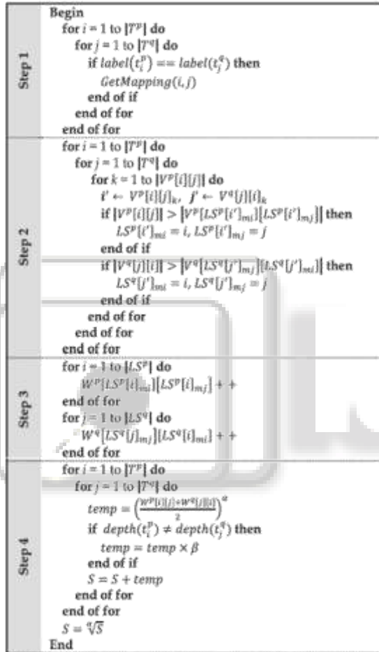
Fig.1. Pseudo code: ref [1].
