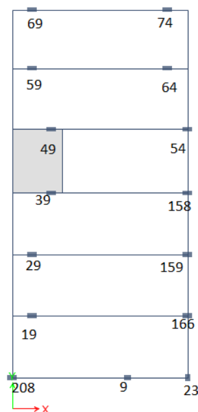
Fig. 2: Footing Node Numbers
