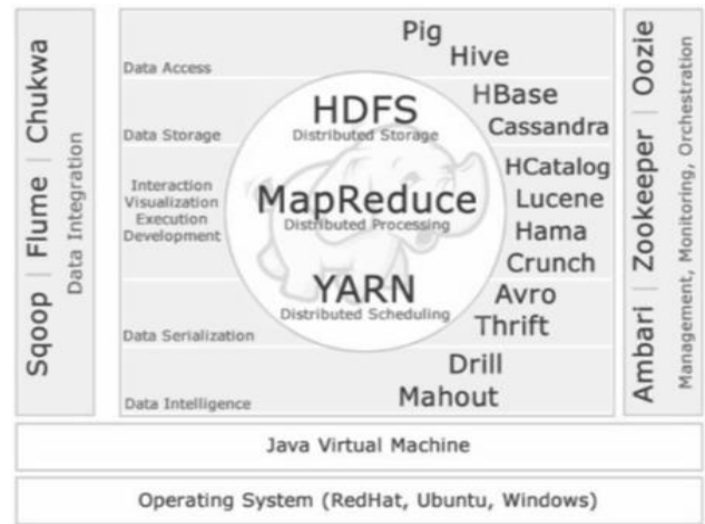
Fig. 2: The image shows the hadoop technology stack
