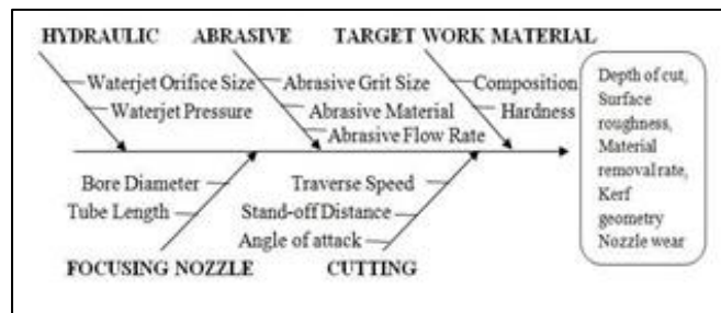
Fig. 2: Process parameters influencing the AWJ cutting process
