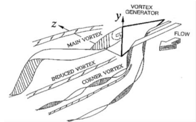
Fig. 1.1: Vortex systems behind a delta winglet
