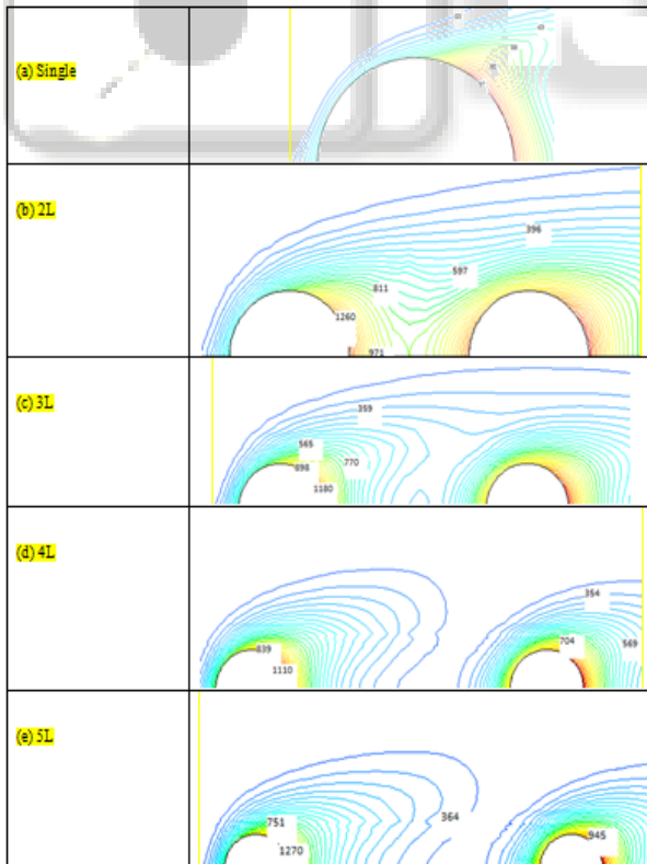
Fig. 4.2: Isotherms (in K) for (a) single and two protrusions with different gap (b) 2L (c) 3L (d) 4L (e) 5L
