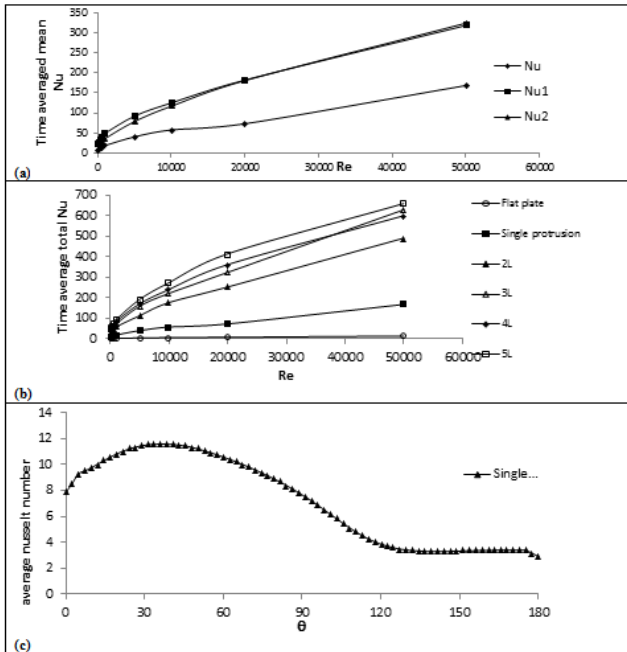
Fig. 4.1: (a) time averaged Nusselt number v/s Reynolds number for 4L and single protrusion, (b) time averaged Nusselt number v/s Reynolds number for flat plate, single protrusion, and two protrusion with gaps of 2L, 3L, 4L and 5L (c): variation of Nusselt number with angular position at Re = 100
