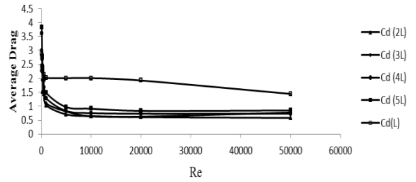
Fig. 4.3: Average drag v/s Reynolds number
