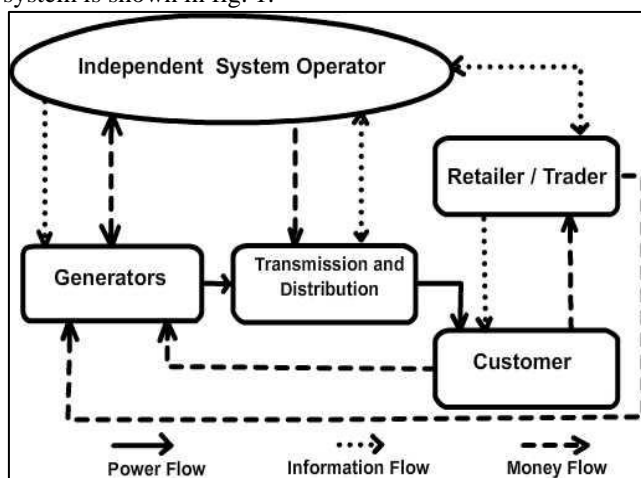
Fig. 1: Deregulated power system
