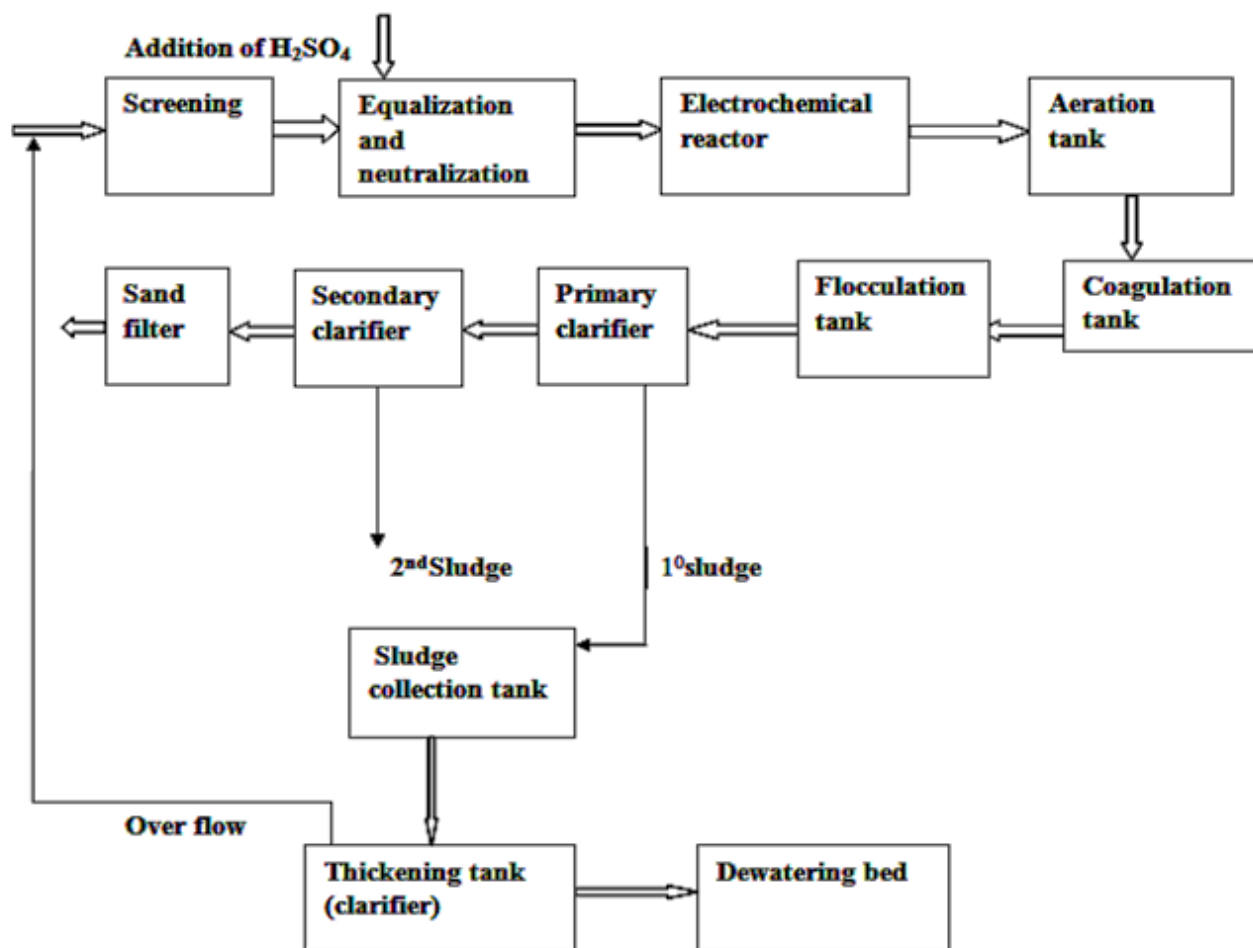
Fig. 2: Flow diagram for Bahir Dar textile waste water treatment plant
