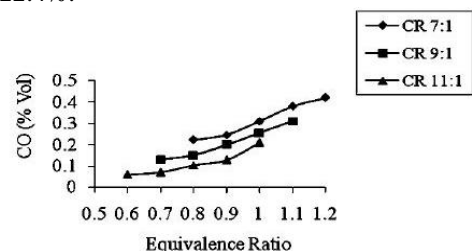
Fig. 7: Fig CO vs Equivalence Ratio (80% of Hydrogen) [7]
