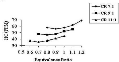
Fig. 6: Fig HC vs Equivalence Ratio (80% of Hydrogen) [7]
