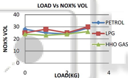
Fig. 4: variation of Nox Against with different load [3]
