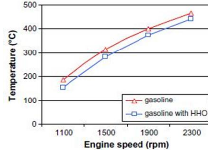
Fig. 1: Engine Speed vs. Temperature [1]
