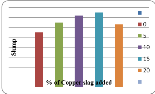
Fig. 7: Variation of slump
