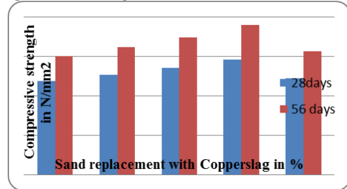
Fig. 4: Compressive strength of concrete by partial replacing sand with copper slag
