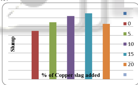
Fig. 2: Variation of slump
