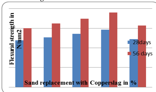
Fig. 6: Flexural strength of concrete by partial replacing sand with copper slag
