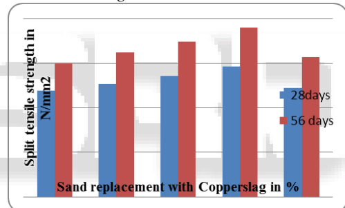
Fig. 5: Split tensile strength of concrete by partial replacing sand with copper slag
