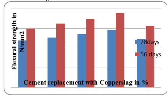
Fig. 10: Flexural strength of concrete by partial replacing cement with copper slag
