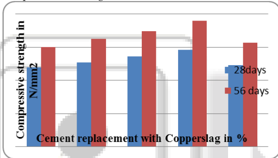
Fig. 8: Compressive strength of concrete by partial replacing cement with copper slag
