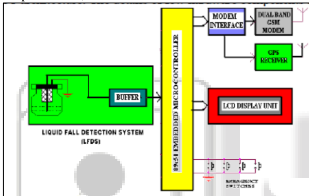
Fig. 3: shows the block diagram of System Unit.
