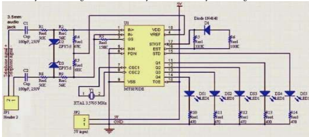
Fig. 3: Connection diagram of DTMF circuit
