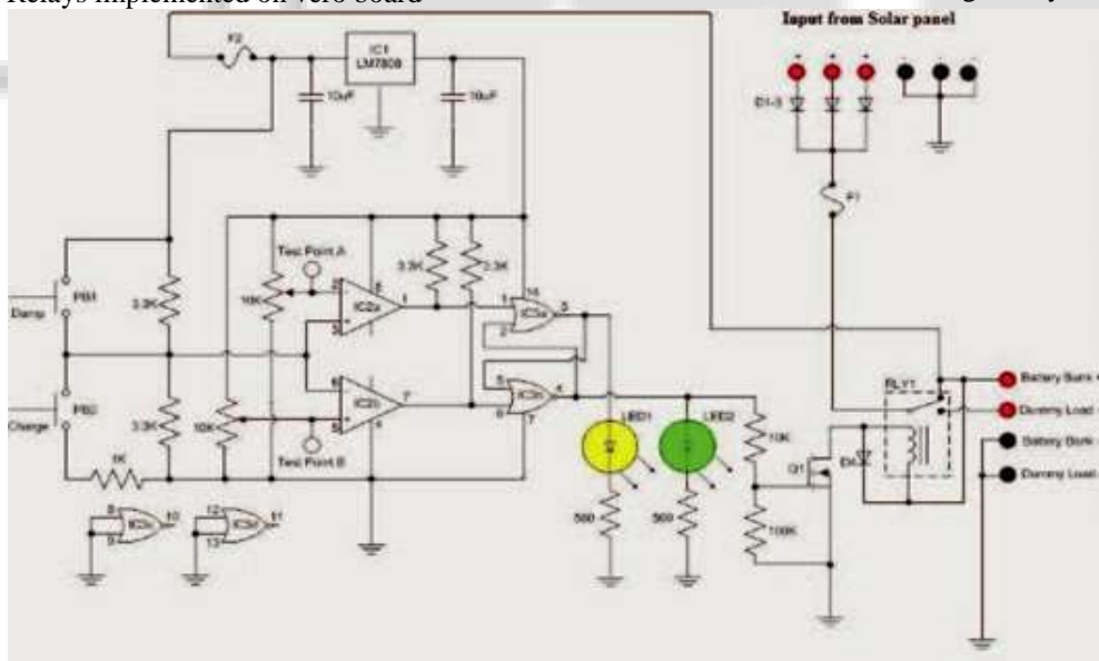
Fig. 5: Solar charge controller circuit diagram
