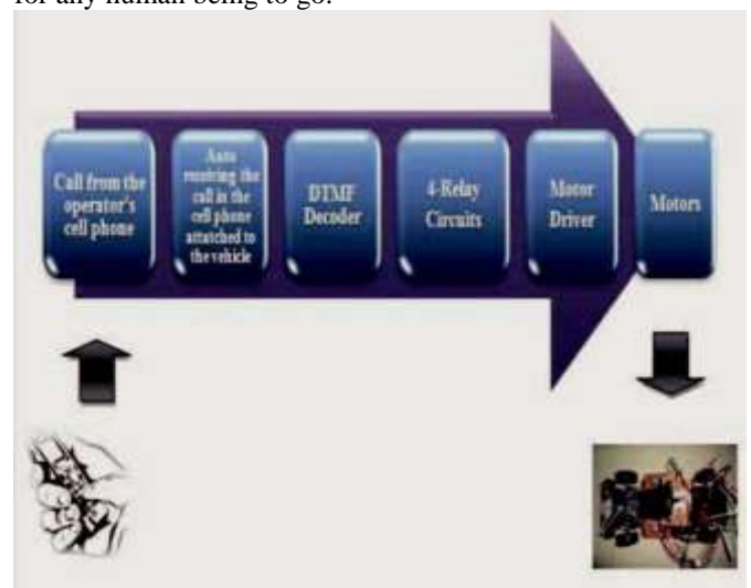
Fig. 1: Block diagram of GSM network controlled vehicle.
