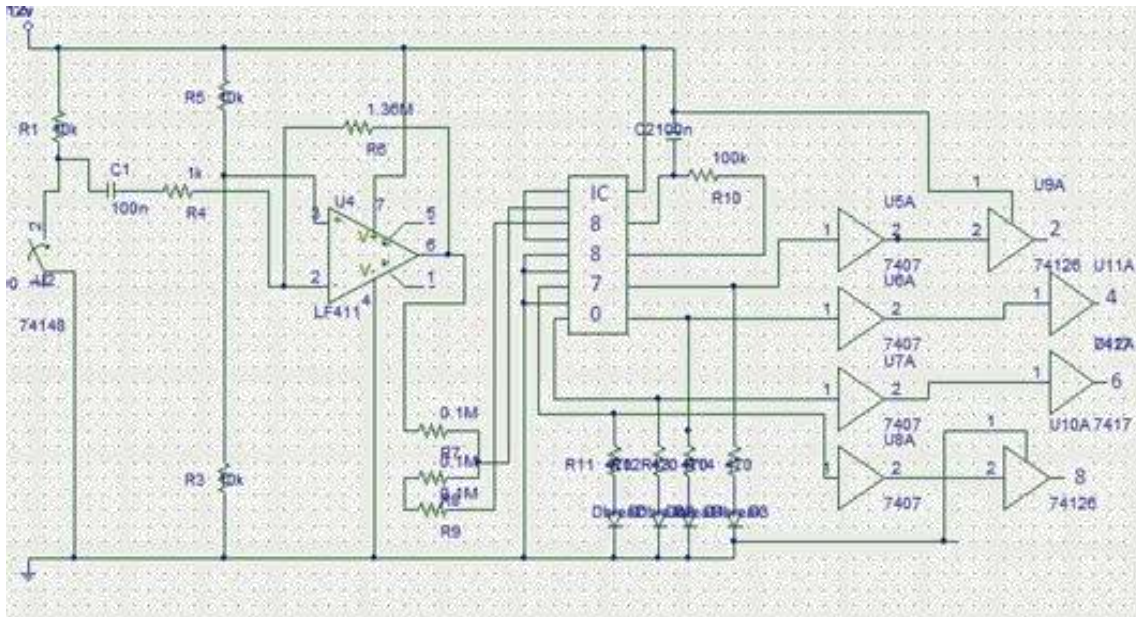
Fig. 2: Circuit diagram of the DTMF operation
