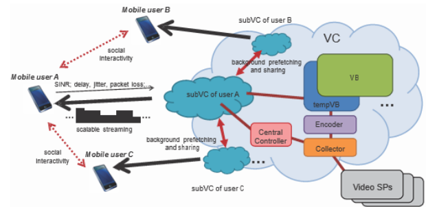
Fig. 1: An illustration of the AMES-Cloud framework
