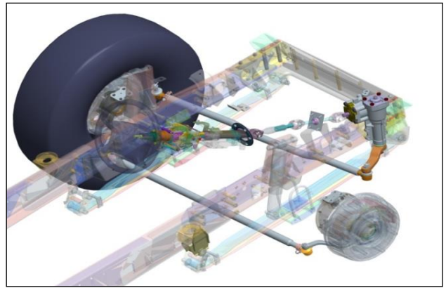
Fig. 12: Final optimized steering linkages CAD image Different iteration are performed on concept 4 to optimize are shown in table 4
