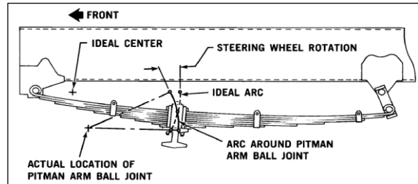
Fig. 3: Bump Steer Phenomena [2]
