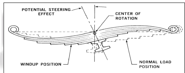
Fig. 4: Spring wind up - Brake Steer Phenomena [2]
