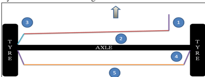
Fig. 11: Optimized Steering Linkages
