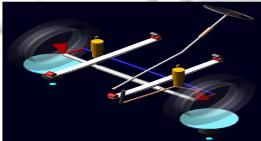
Fig. 6: ADAMS model for Bump and Brake steer calculations
