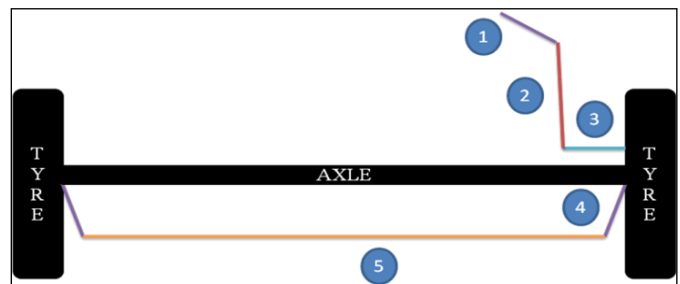
Fig. 8: Concept 1, 2 Steering Linkages
