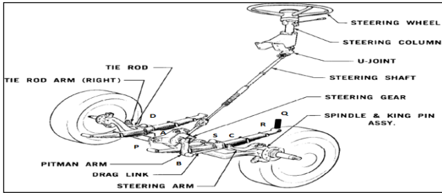
Fig. 5: Typical Steering system and hard points [2]
