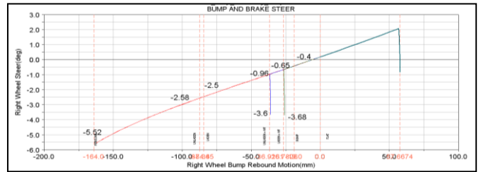
Fig. 7: Brake and Bump steer graph
