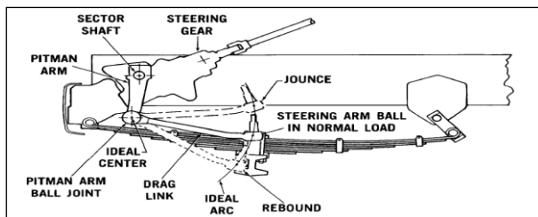
Fig. 2: Ideal location of Pitman arm ball joint [2]
