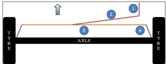
Fig. 9: Concept 3 Steering Linkages
