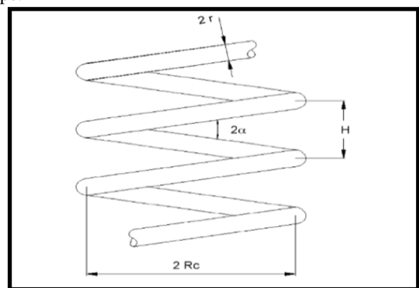
Fig. 2: Basic geometry of a helical pipe.
