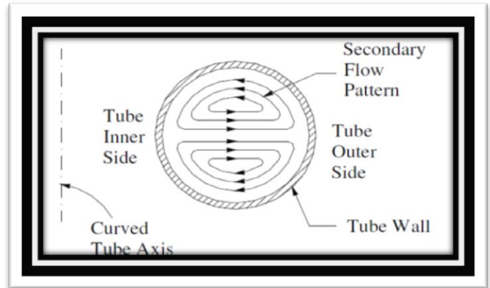
Fig. 1: Fluid flow in curved pipes
