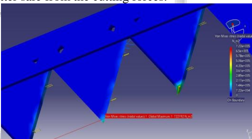
Fig. 15: Force Analysis on the Cutter Blade
