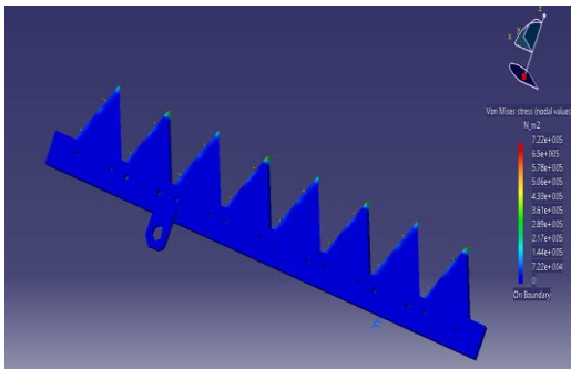
Fig. 14: Force Analysis on the Cutter Blade
