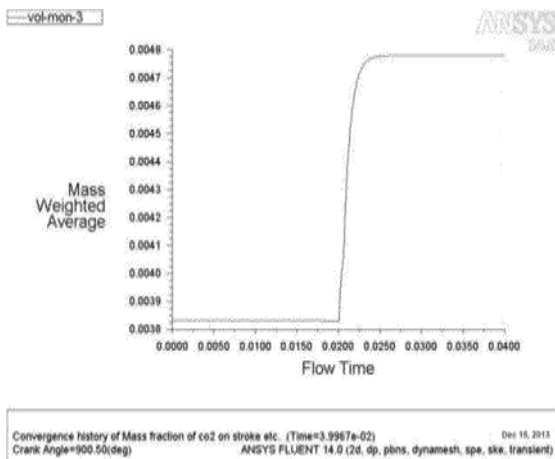
Fig.6. Mass fraction of CO 2
