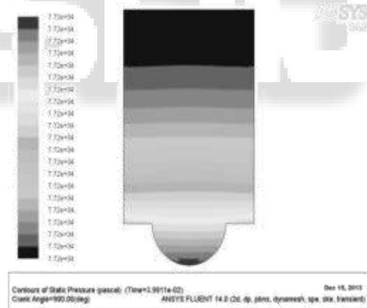
Fig.4. Contours of static pressure
