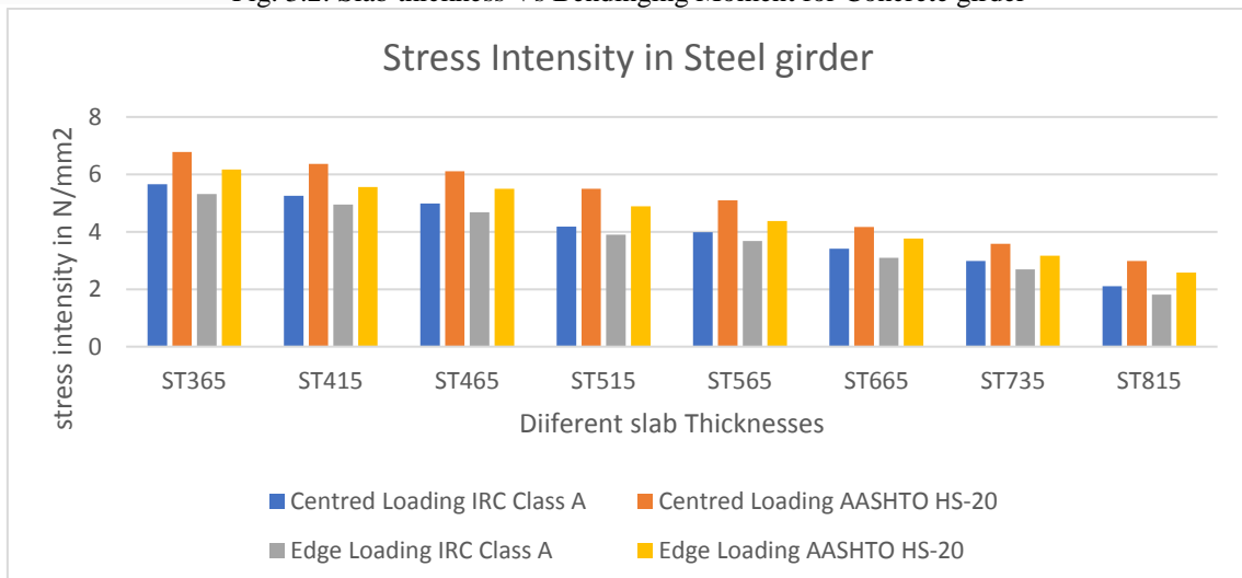
Fig. 4.1: Slab thickness Vs Stress intensity in steel girder
