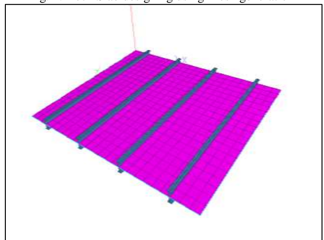
Fig. 2: 3D render view of Deck Slab
