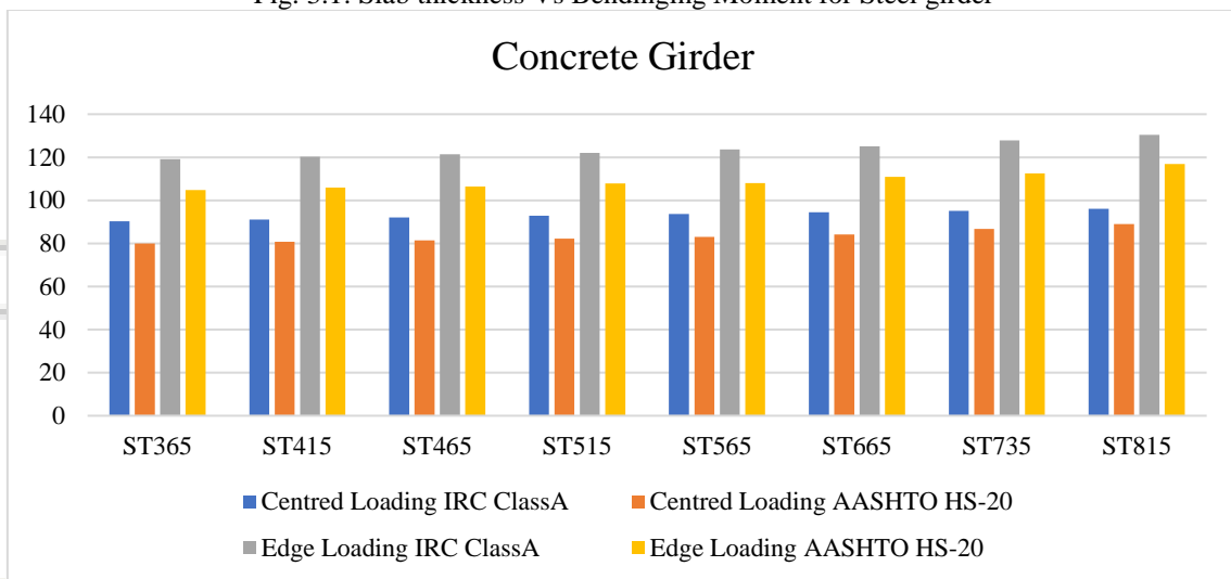
Fig. 3.2: Slab thickness Vs Bending Moment for Concrete girder
