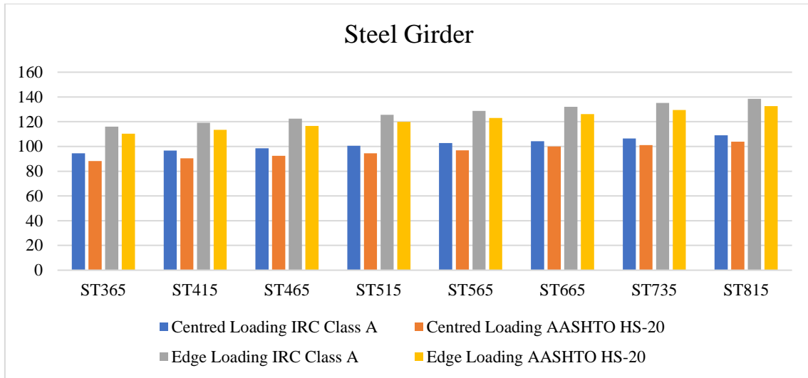
Fig. 3.1: Slab thickness Vs Bending Moment for Steel girder
