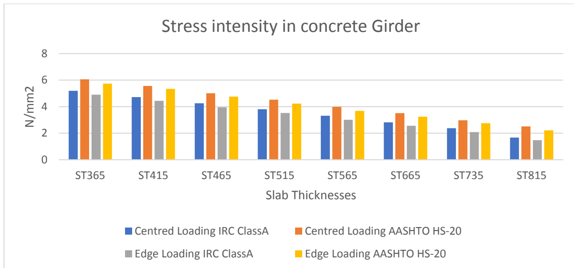
Fig. 4.2: Slab thickness Vs Stress intensity in Concrete girder
