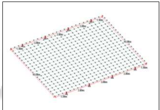
Fig. 1: Deck Slab designing using Mesh generation
