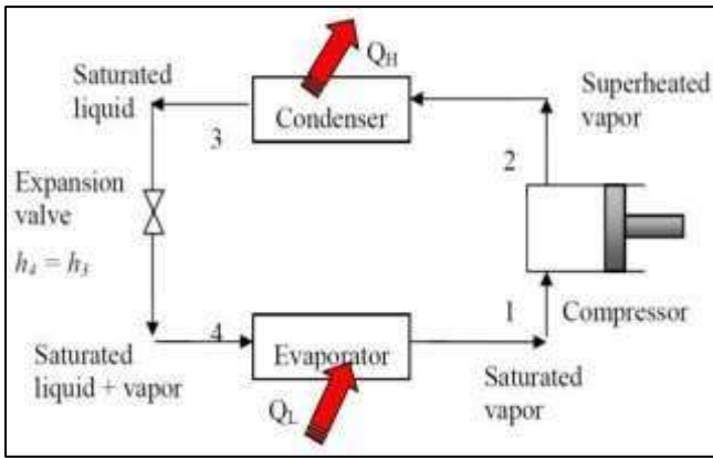
Fig. 1: Schematic diagram of VCRS
