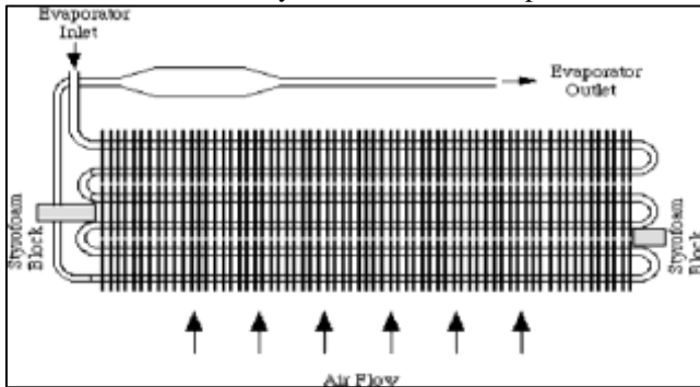
Fig. 5: Arrangement of Evaporator
