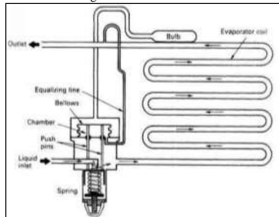
Fig. 4: Thermal expansion valve
