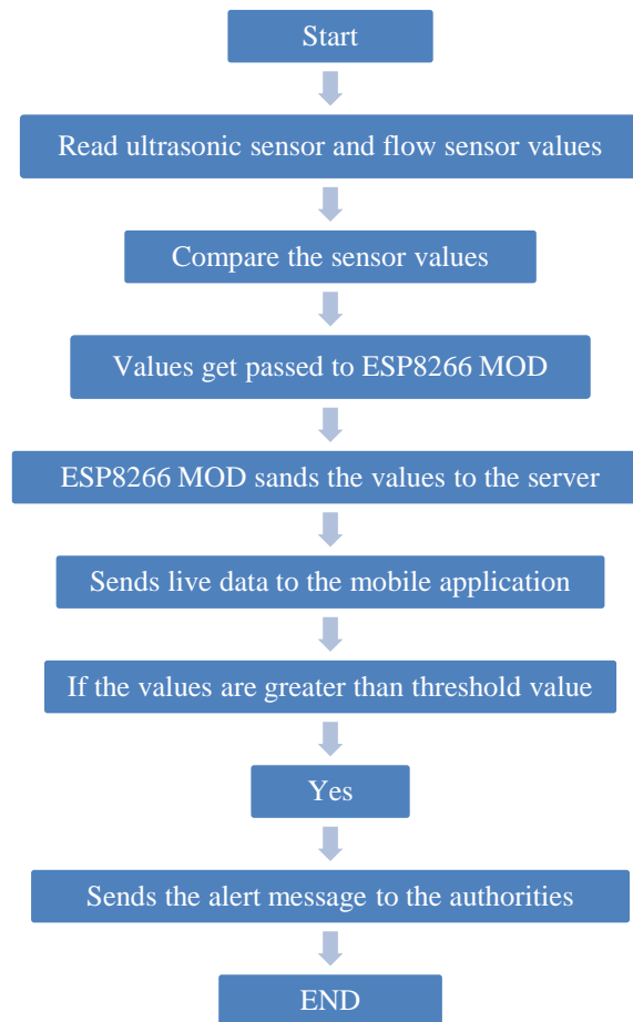
Fig. 3: Methodology of system
