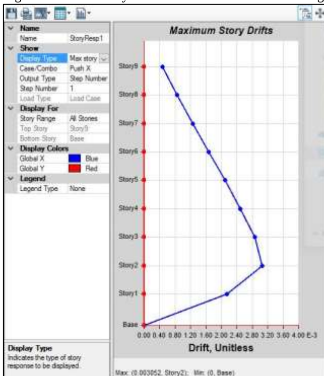
Fig. 3: Maximum story drift for the third case of building.
