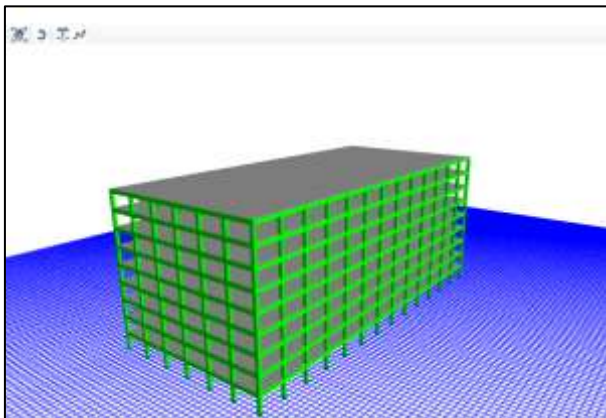
Fig. 1: 3D figure of the building frame to be analyzed using different combinations of columns.
