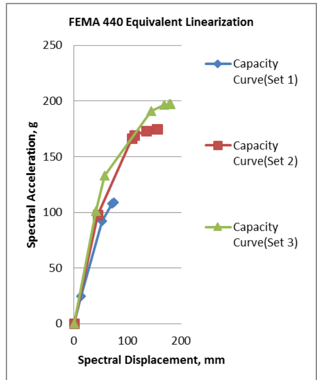
Fig. 2: Capacity Curves for the three cases of buildings
