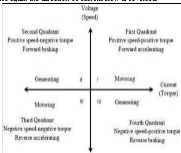
Fig. 4: Four Quadrant Operation of a DC Motor
