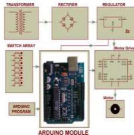
Fig. 1: Block Diagram for four Quadrant DC Motor Speed control by using Arduino
