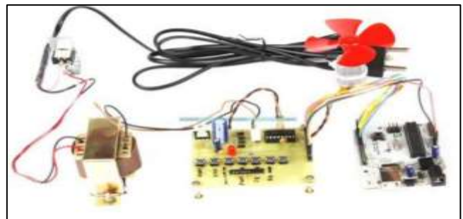
Fig. 5: Practical Implementation of Speed Control DC Motor
