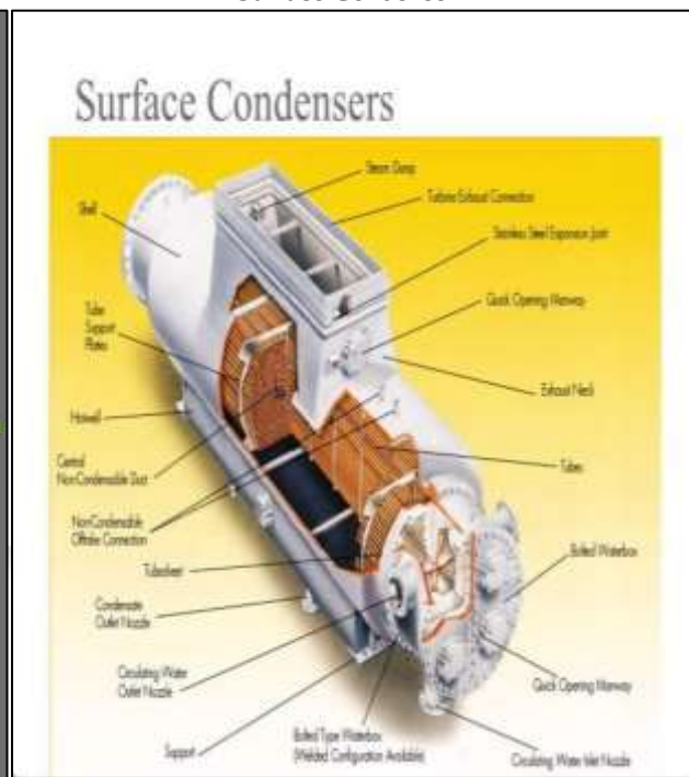
Surface Condenser
