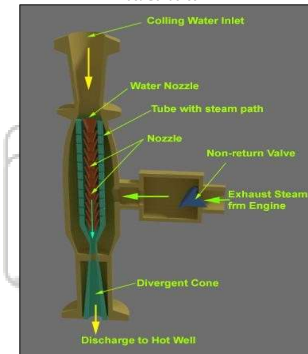
Jet condenser
