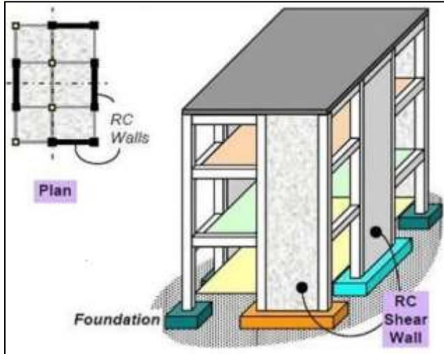
Fig. 1.3: plan and elevation of shear wall
