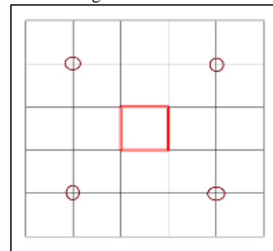
Case 5: removing the 4 columns in the ground floor with shear wall in centrally core (Box type)
