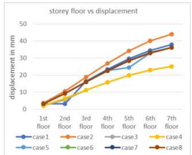
Fig. 3.2: displacement in mm
