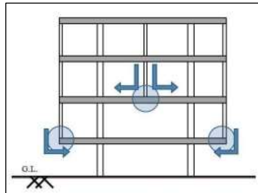
Fig. 1.1: load distribution of floating column
