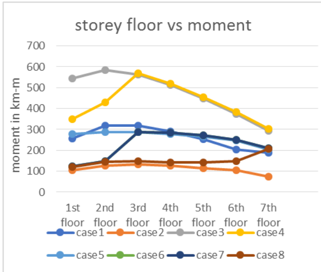
Fig. 3.3: moment in km-m
