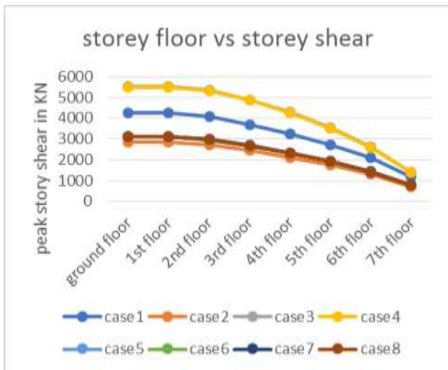
Fig. 3.4: storey shear (KN)
