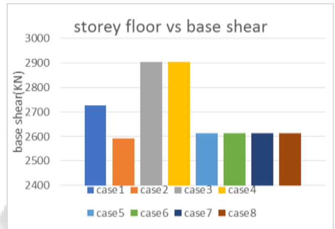
Fig. 3.1: base shear (KN)
