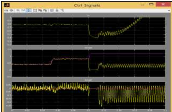
Fig. 9: Output waveform of the AC/DC Three Level Control Signal PWM Converter
