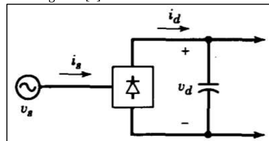
Fig. 1: Block diagram of a rectifier
