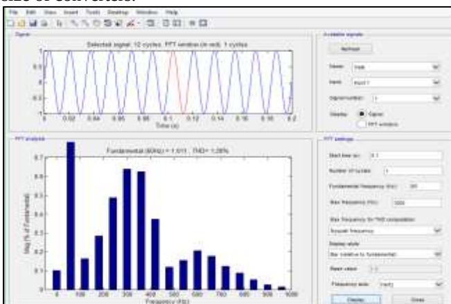
Fig. 10: Total Harmonic Distortion
