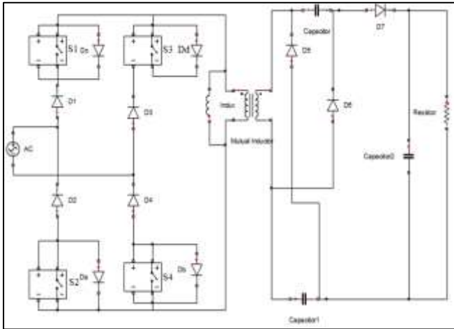
Fig. 4: Circuit of Proposed Converter using Switching Capacitor Technique
