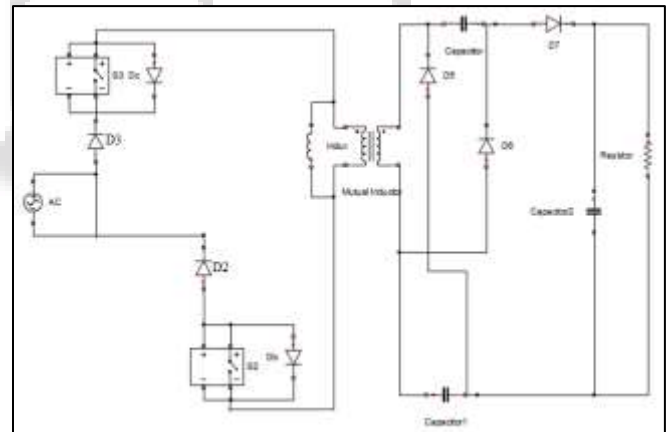
Fig. 7: Circuit operation in mode-II
