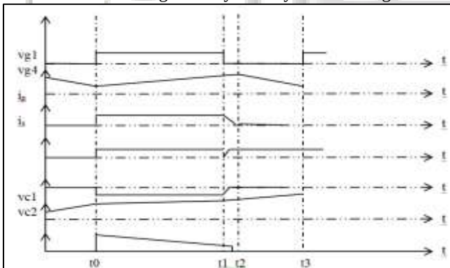
Fig. 5: Waveforms of AC-DC Converter using Switching Capacitor Technique
