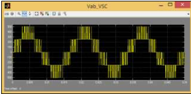
Fig. 8: Output waveform of the AC/DC Three Level PWM Converter
