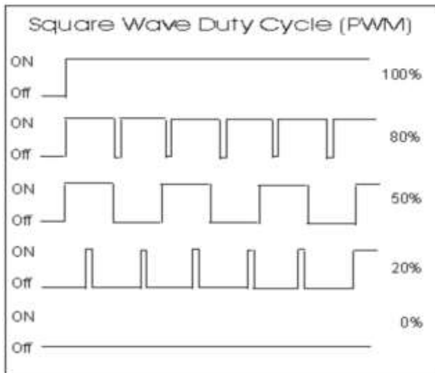
Fig. 2: Pulse Width Modulation
