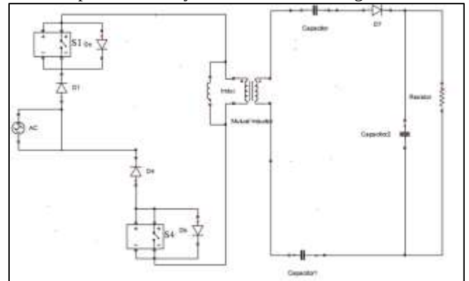
Fig. 6: Circuit operation in mode-I
