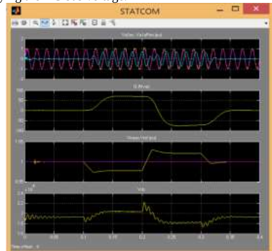
Figure 4: Output Waveform of the STATCOM
