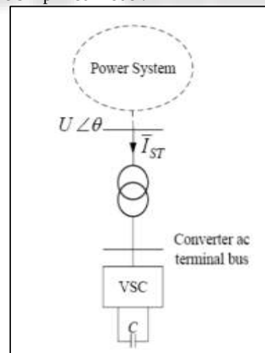
Fig. 1: Line diagram of STATCOM
