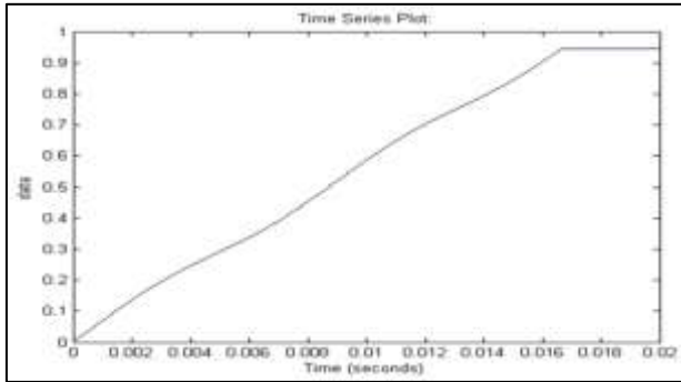
Fig. 8: Voltage v/s time plot of bus-1 of IEEE 14-bus system with FLC based STATCOM
