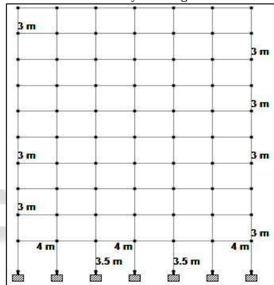
Fig. 2: Represents Elevation of conventional slab system for 10 storey building.
