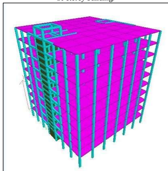
Fig. 3: 3-D model of model 1 of Flat slab without shear wall.
