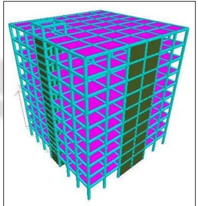
Fig. 8: 3-D model of model 6 of Conventional slab with shear wall in Z- direction.
