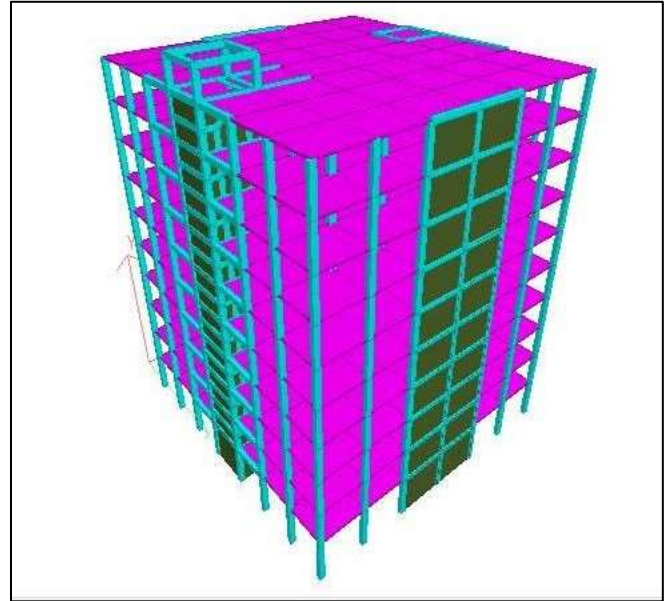
Fig. 7: 3-D model of model 5 of Flat slab with shear wall in Z-direction.
