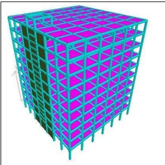
Fig. 6: 3-D model of model 4 of Conventional slab with shear wall in X-direction.
