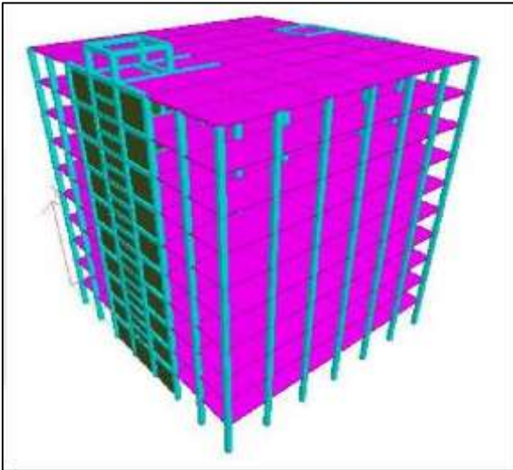
Fig. 5: 3-D model of model 3 of Flat slab with shear wall in X-direction.
