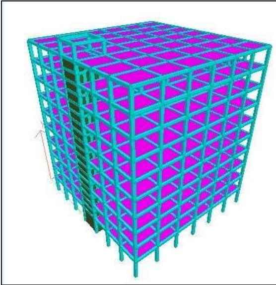
Fig. 4: 3-D model of model 2 of Conventional slab without shear wall.
