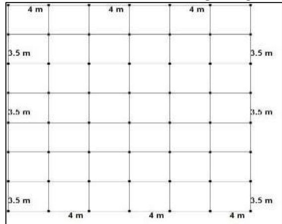
Fig. 1: Represents plan area of conventional slab system for 10 storey Building.
