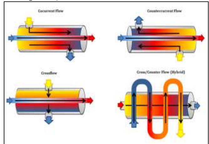
Fig. 2: Types of Heat Exchanger on Basis of Flow
