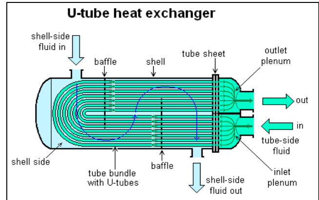
Fig. 1: Diagram of Shell & Tube Heat Exchanger
