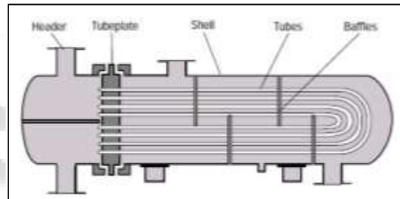
Fig. 6: U-Tube Shell & Tube Heat Exchanger
