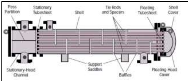
Fig. 8: Fixed Tube Shell & Tube Heat Exchanger
