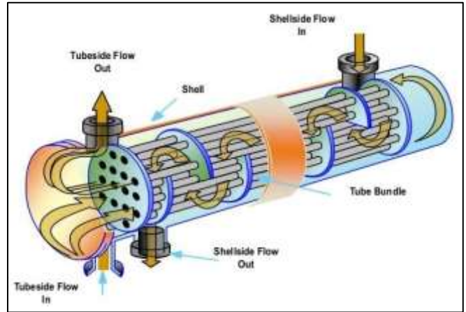
Fig. 5: Shell & Tube Heat Exchanger
