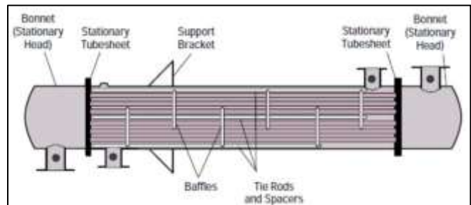
Fig. 7: Fixed Tube Shell & Tube Heat Exchanger
