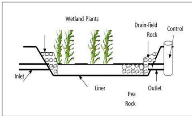
Fig. 5: A Subsurface Flow Constructed Wetland Sketch Vymazal (2001)
