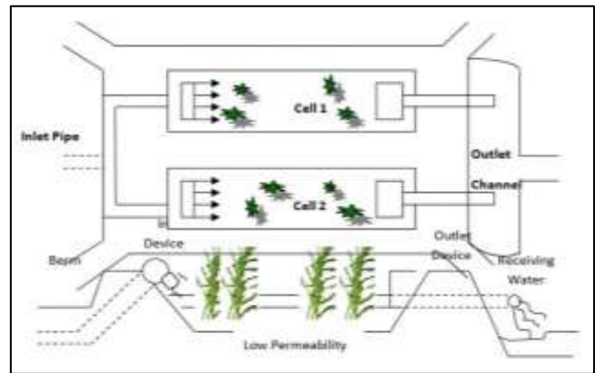
Fig. 1: Plan and Profile of a Typical Free Water Surface Wetland
