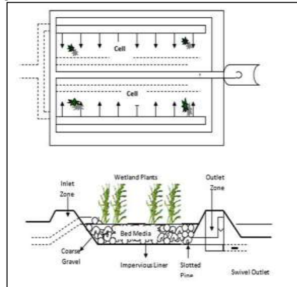
Fig. 3: A Sectional View of Wetland Controls and Liner Davis (1995).
