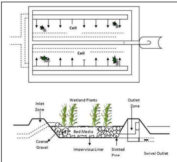
Fig. 2: Plan and Cross-Sectional View of a Subsurface Flow Wetland Wallace and Knight (2006).
