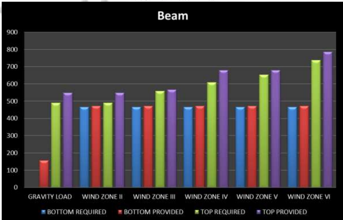
Fig. 7: Area of Steel in Beams
