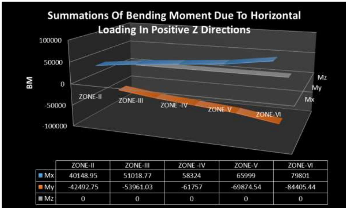
Fig. 6: Bending Moment Due To Horizontal Loading In Positive Z Directions:-
