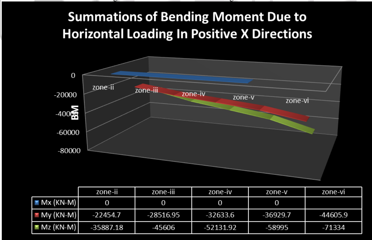
Fig. 5: Bending Moment Due to Horizontal Loading in Positive X Directions:-
