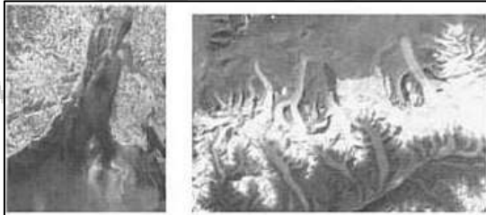
Fig. 1: Example of a remotely sensed image of (a) delta of river Ganges, (b) Glacier flow in Bhutan Himalayas
