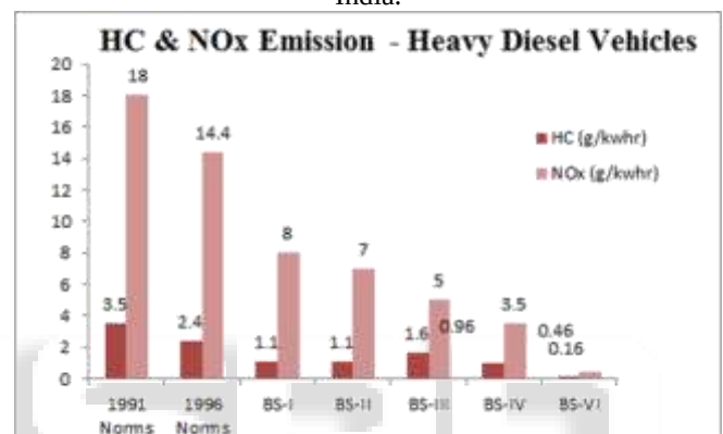
Fig. 6: Maximum Allowable HC and NO x emission from Heavy Diesel Vehicles according to various emission standards of India.
