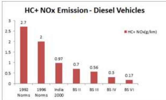
Fig. 4: Maximum Allowable HC+NO x emission from passenger cars powered by diesel according to various emission standards of India.
