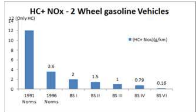
Fig. 10: Maximum Allowable HC + NOx emission from 2 wheeled gasoline powered vehicles according to various emission standards of India
