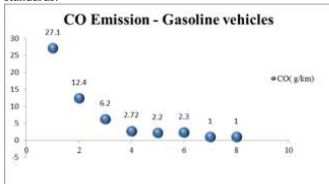
Fig. 1: Maximum Allowable CO emission from passenger cars powered by petrol according to various emission standards of India.
