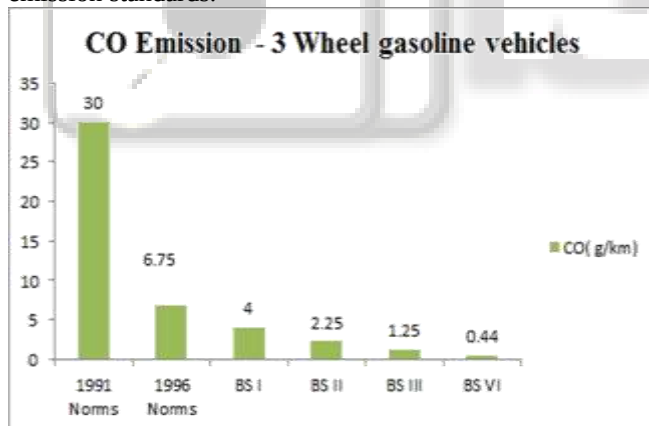
Fig. 9: Maximum Allowable CO emission from 3 wheeled gasoline powered vehicles according to various emission standards of India
