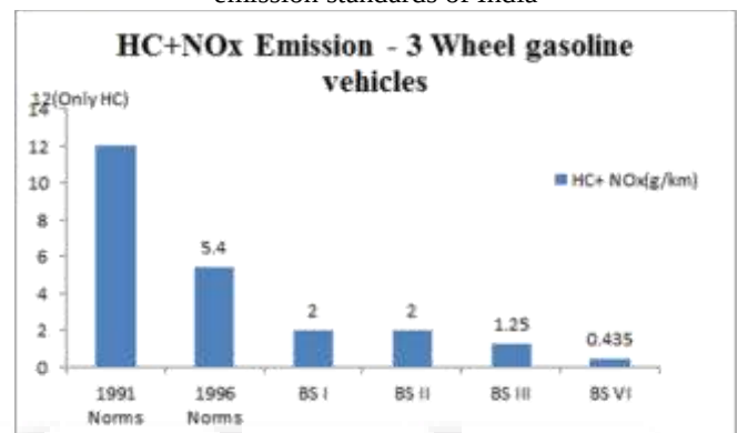
Fig. 11: Maximum Allowable HC + NOx emission from 3 wheeled gasoline powered vehicles according to various emission standards of India
