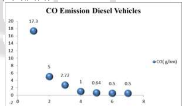
Fig. 2: Maximum Allowable CO emission from passenger cars powered by diesel according to various emission standards of India
