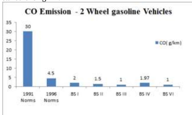
Fig. 8: Maximum Allowable CO emission from 2 wheeled gasoline powered vehicles according to various emission standards of India
