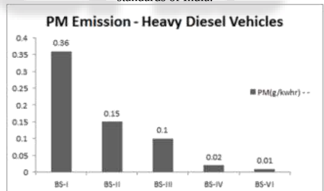
Fig. 7: Maximum Allowable PM emission from Heavy Diesel Vehicles according to various emission standards of India.
