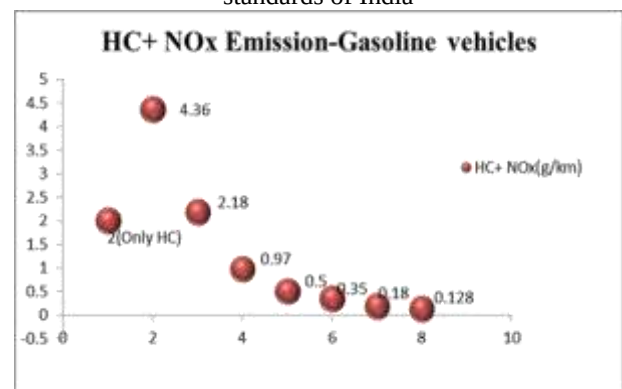
Fig. 3: Maximum Allowable HC+NOx emission from passenger cars powered by petrol according to various emission standards of India.
