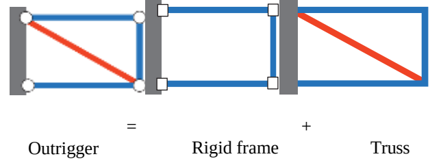
Fig. 1.3.3: Simplified mathematical model of outriggers.
