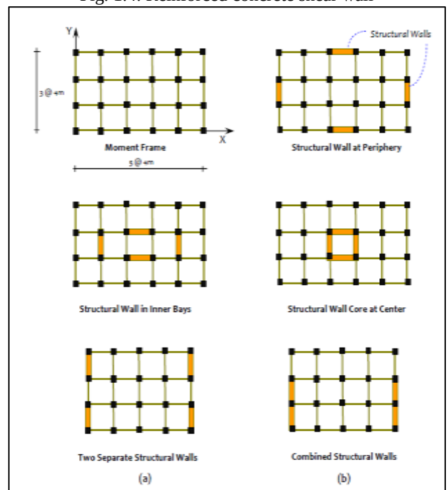
Fig. 1.4.1: Position of shear walls in a moment resisting frame building
