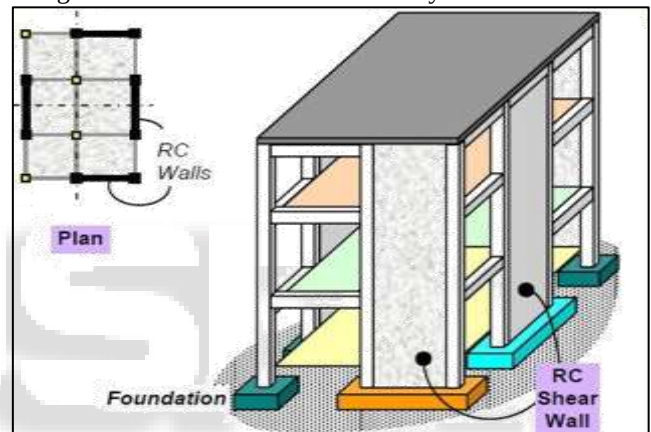
Fig. 1.4: Reinforced concrete shear wall
