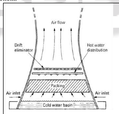
Fig. 2.1: Natural draft cooling tower
