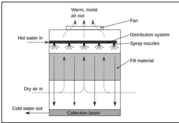
Fig. 2.2: Mechanical Draft Cooling Tower
