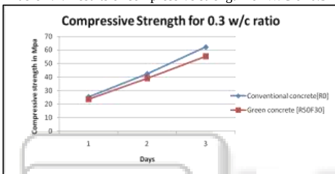
Fig. 7.1: Variation of compressive strength with age for W/C of 0.3
