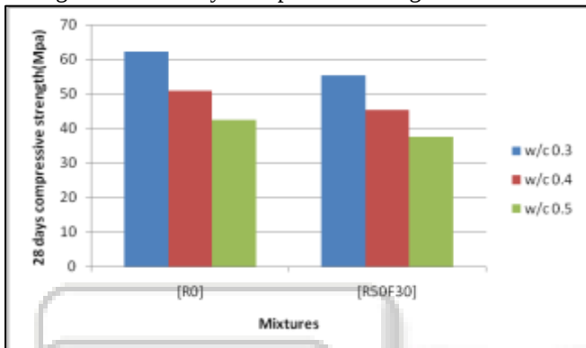
Fig. 7.6: Twenty eight days compressive strength of concrete
