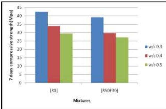
Fig. 7.5: Seven days compressive strength of concrete
