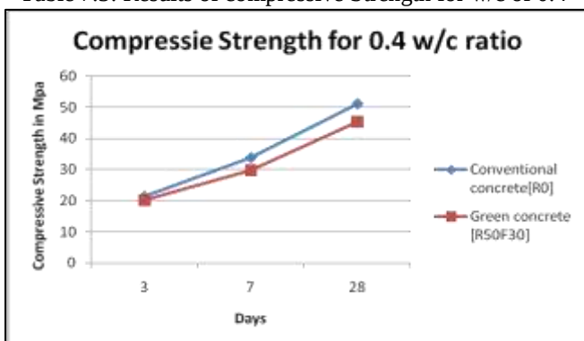
Fig. 7.2: Variation of compressive strength with age for W/C of 0.4
