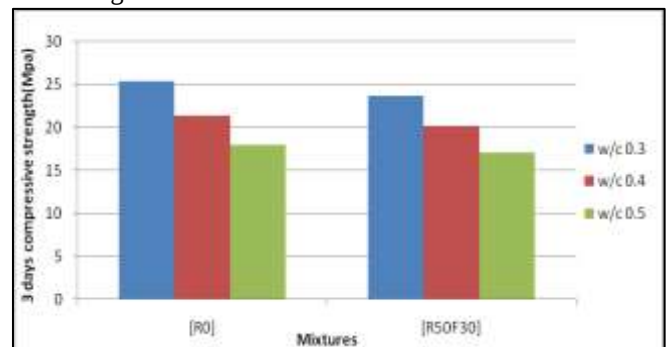
Fig. 7.4: Three days compressive strength of concrete
