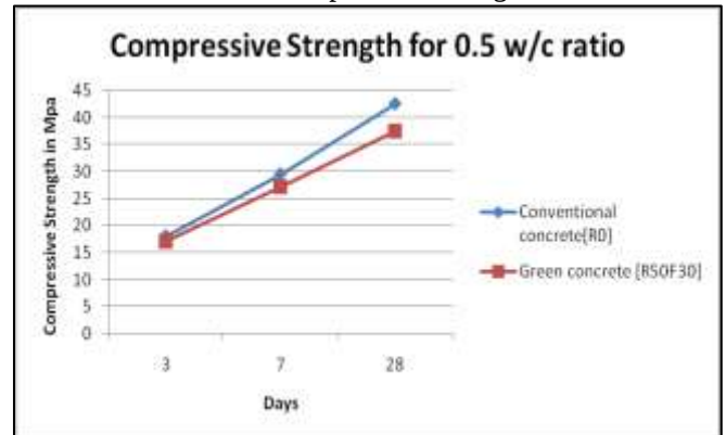
Fig. 7.2: Variation of compressive strength with age for W/C of 0.5
