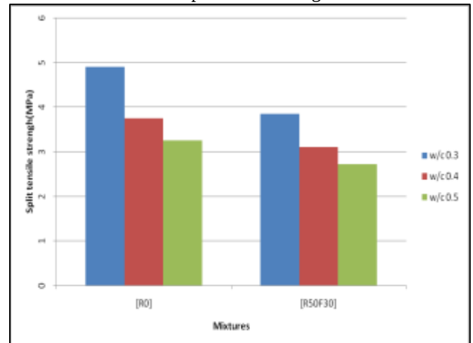
Fig. 7.7: Twenty eight days split tensile strength
