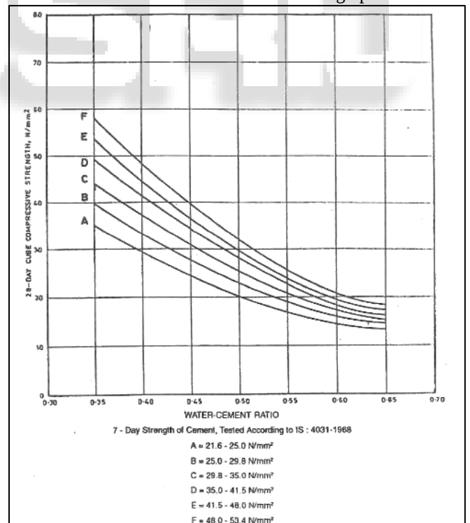
Fig. 2: Concrete Compressive Strength vs. Water Cement Ratio
