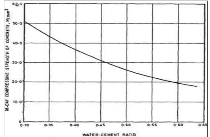
Fig. 1: Selection of Water-Cement Ratio for Concrete Mix Design
