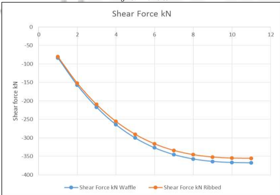
Fig. 16: Shear Force
