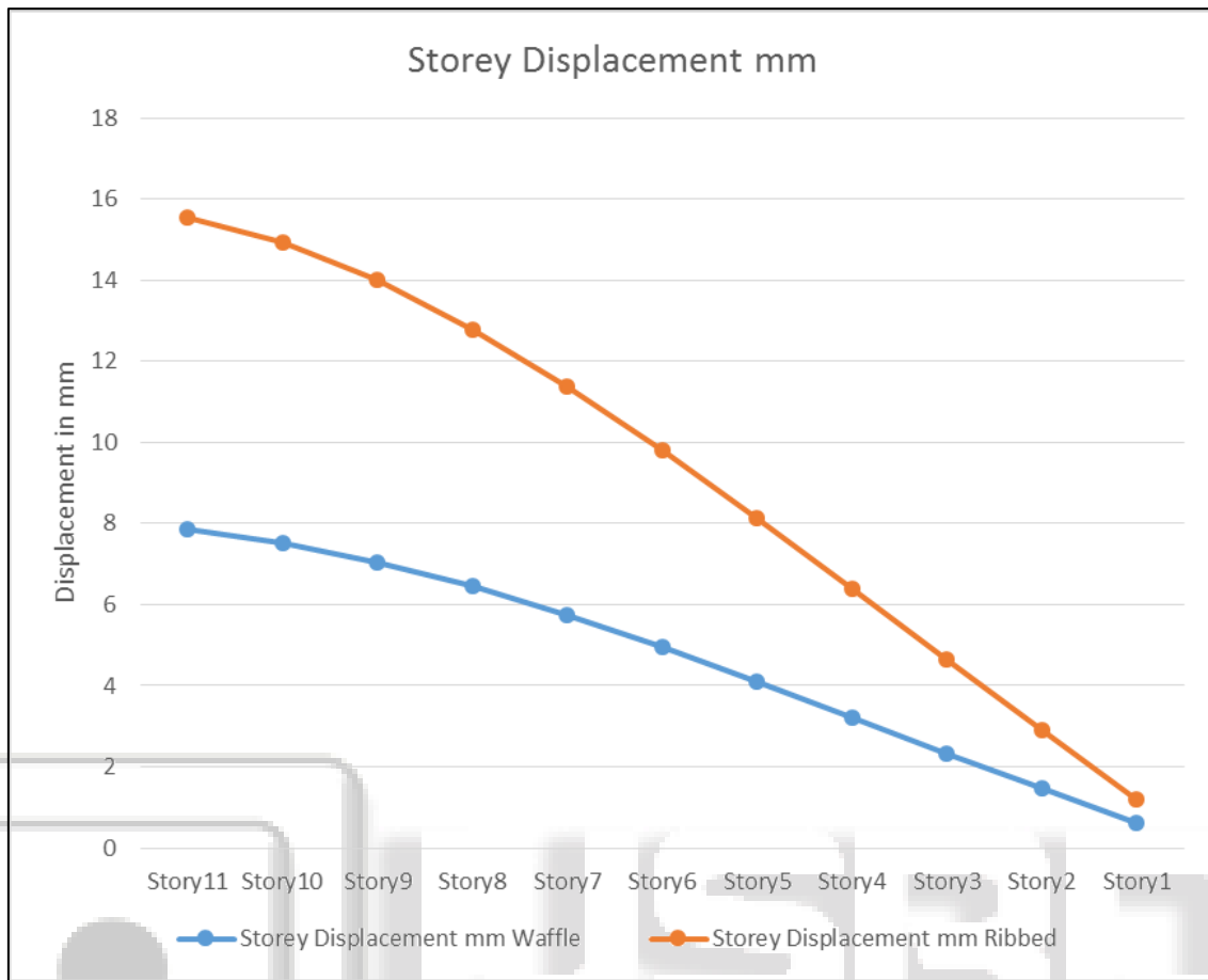
Fig. 13: Storey Displacement
