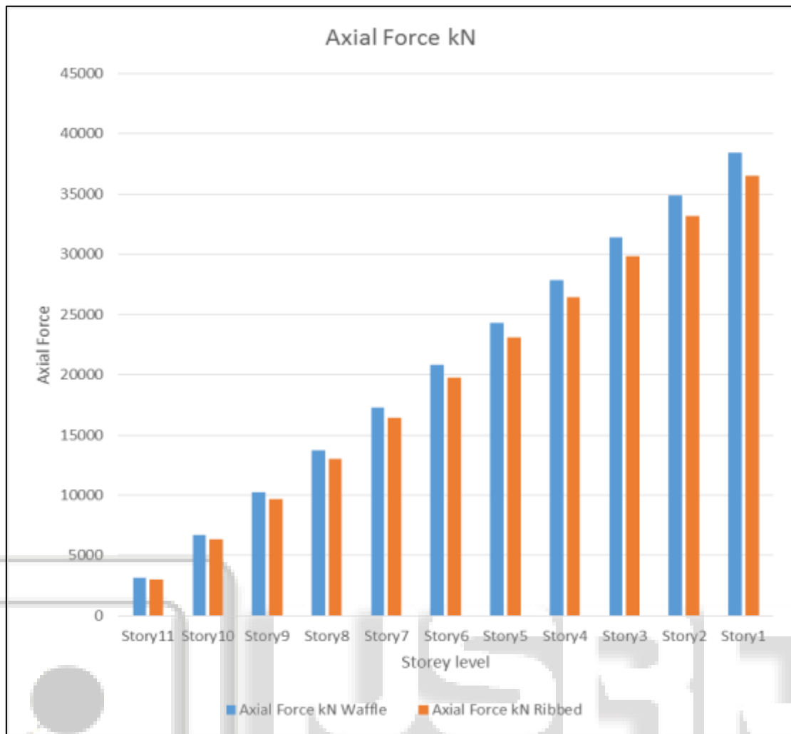
Fig. 15: Axial force
