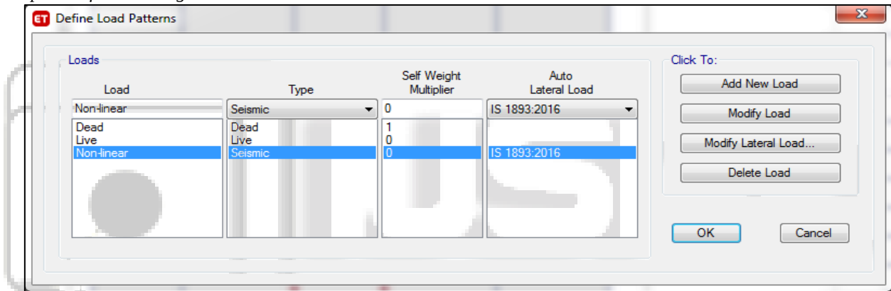
Fig. 10: Loading Conditions
