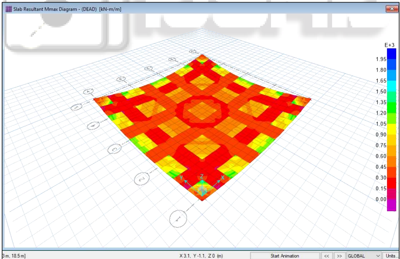
Fig. 8: Slab configuration
