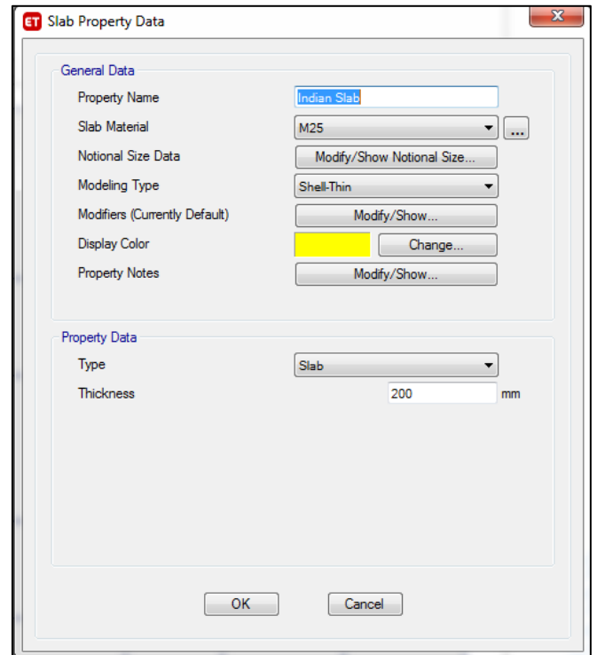
Fig. 6: Sectional data
