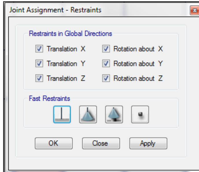
Fig. 9: End conditions
