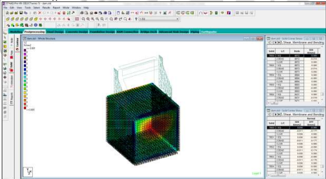
Fig. 8: Soil Interaction
