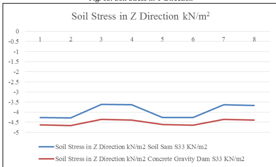
Fig. 16: Soil Stress in Z Direction
