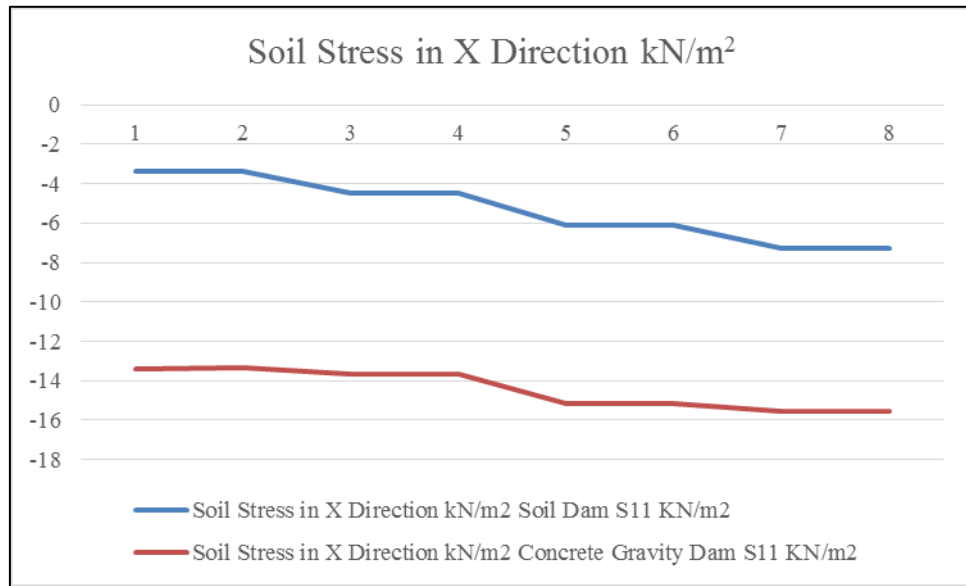
Fig. 14: Soil Stress in X Direction
