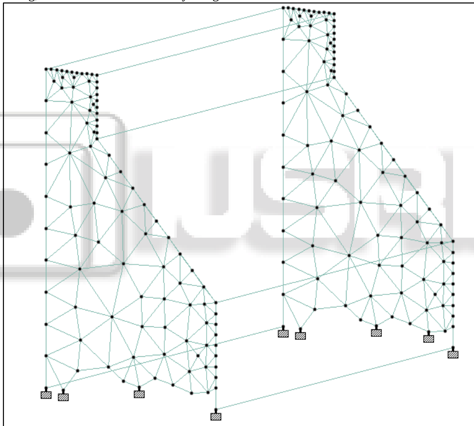
Fig. 2: Modelling of Dam using Staad wizard
