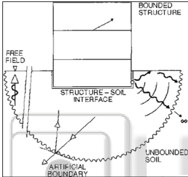
Fig. 1: Soil Interaction
