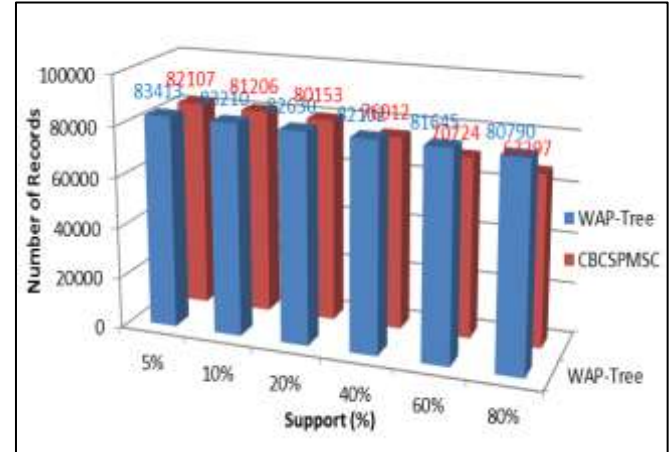
Fig. 8: Comparison of WAP-Tree and CBCSPMSC Algorithm with different support (By using Record-Size 6050)
