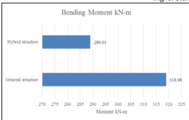
Fig. 9: Bending Moment
