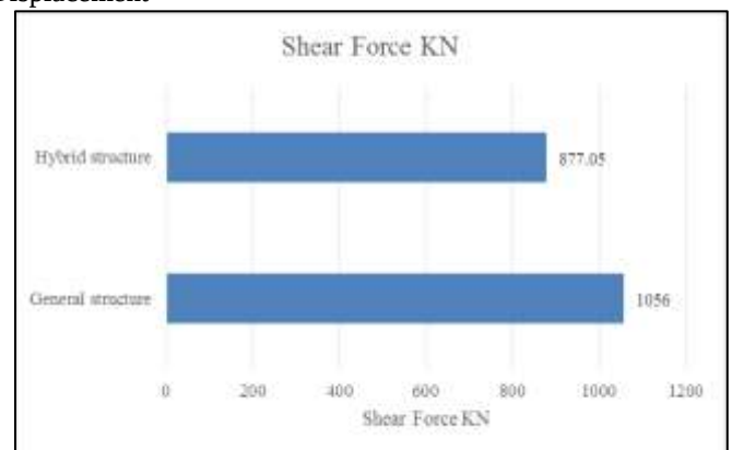
Fig. 10: Shear Force
