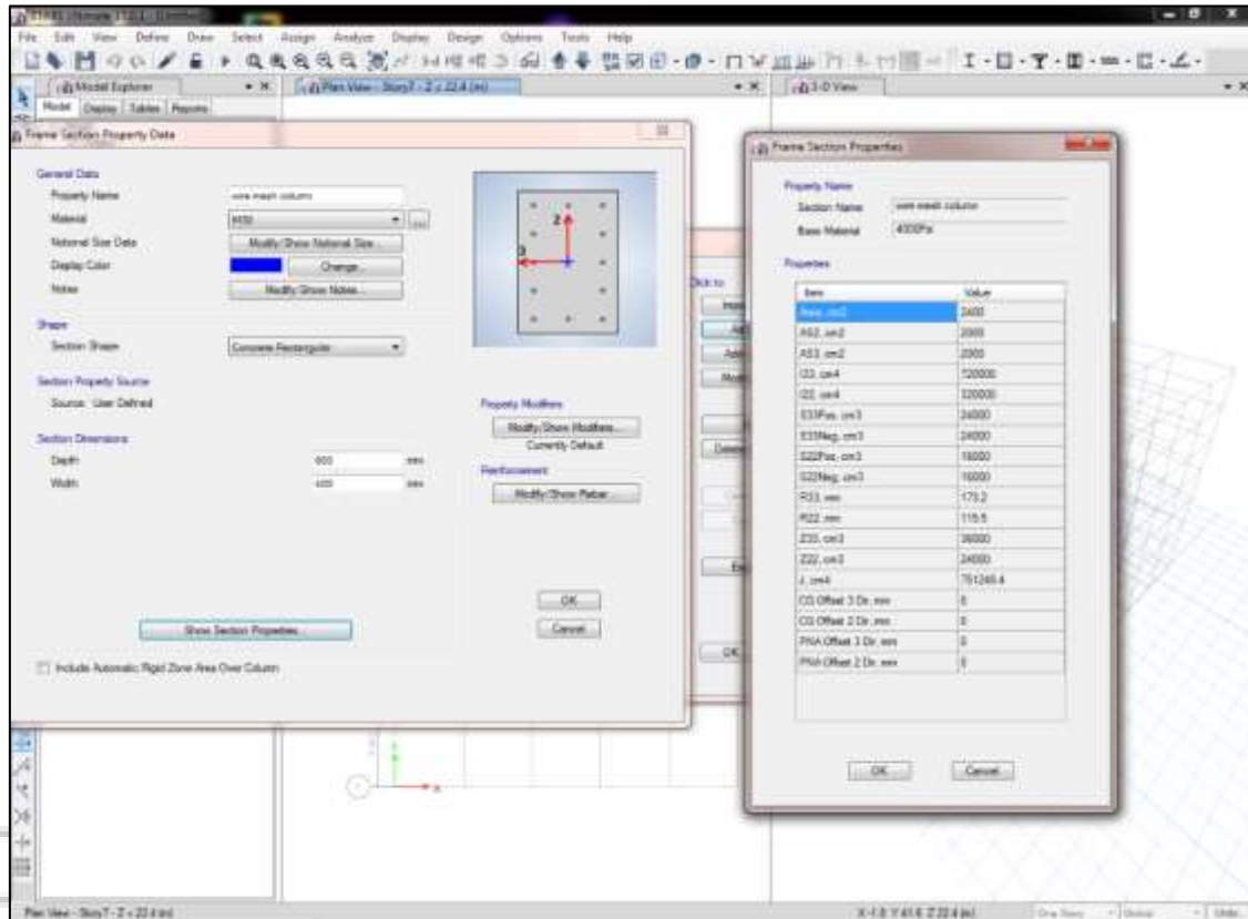
Fig. 2: Ferroconcrete material sections
