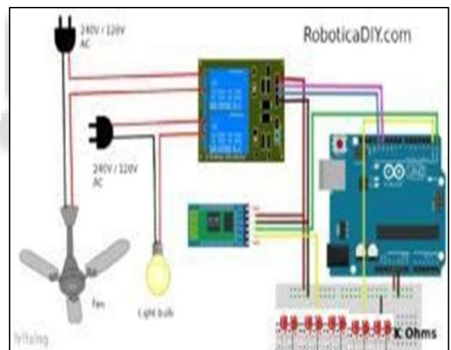
Fig. 3: Circuit model of project
