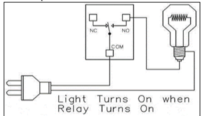
Fig. 7: connection for relay and AC bulb
