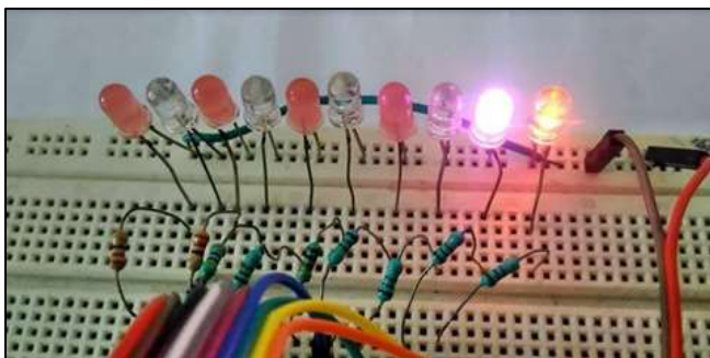
Fig. 6: LEDs glow as per attention
