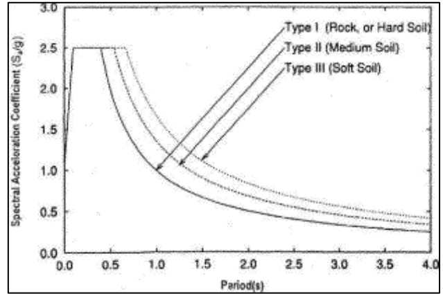
Fig. 3: Design spectrum as per IS: 1893-2002
