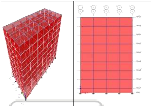
Fig. 6: 3D view and elevation of eight storeyed building
