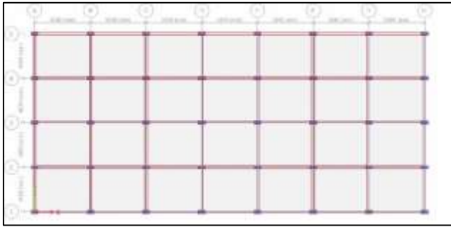
Fig. 5: Plan layout of model (G+15)
