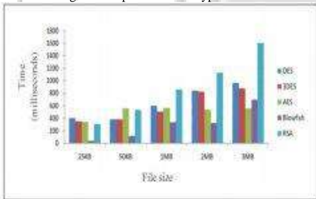
Fig. 8: Comparison of decryption time
