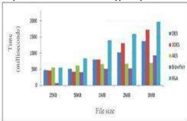
Fig. 7: Comparison of encryption time
