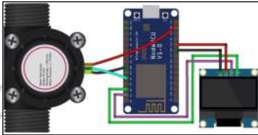
Fig. 4: Hardware Connectivity to Nodemcu
