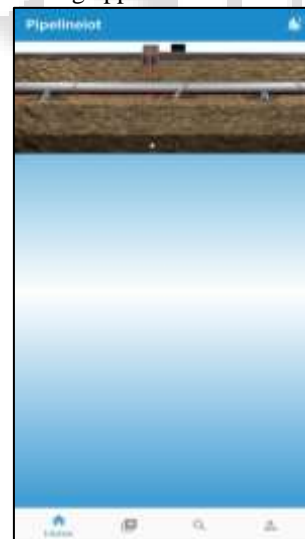
Fig. 5.1: Home Screen
